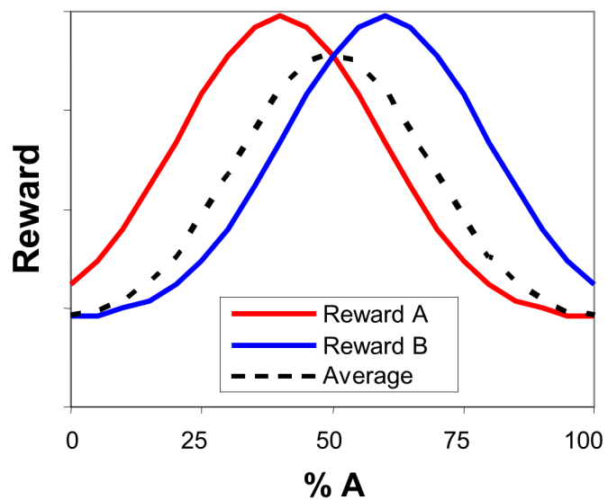
Converging Gaussians
