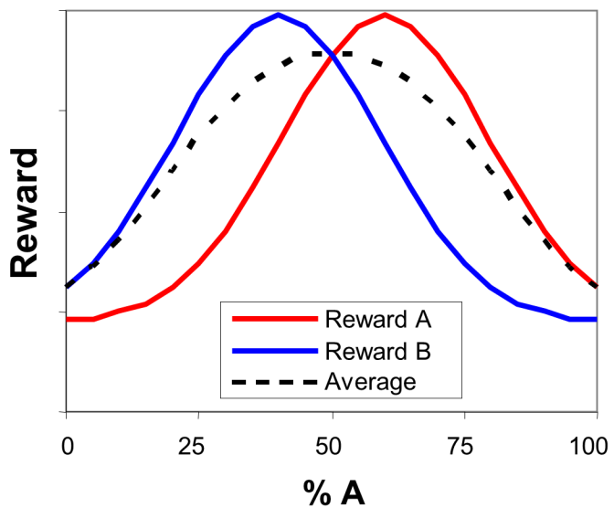
Diverging Gaussians
